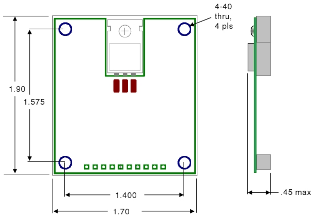
5538 Single Channel YIG Driver
